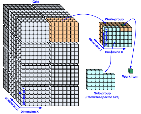
Figure 1. The OpenCL execution hierarchy.
