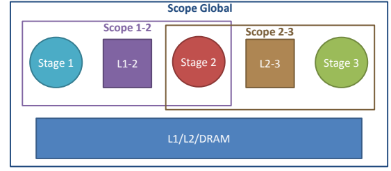
Figure 8. Architecture and scope layout of a possible programmable pipeline.
